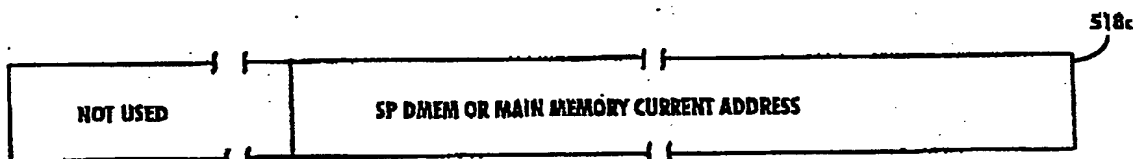
Fig. 21C DP CMD DMA CURRENT ADDRESS REGISTER (R/W)
